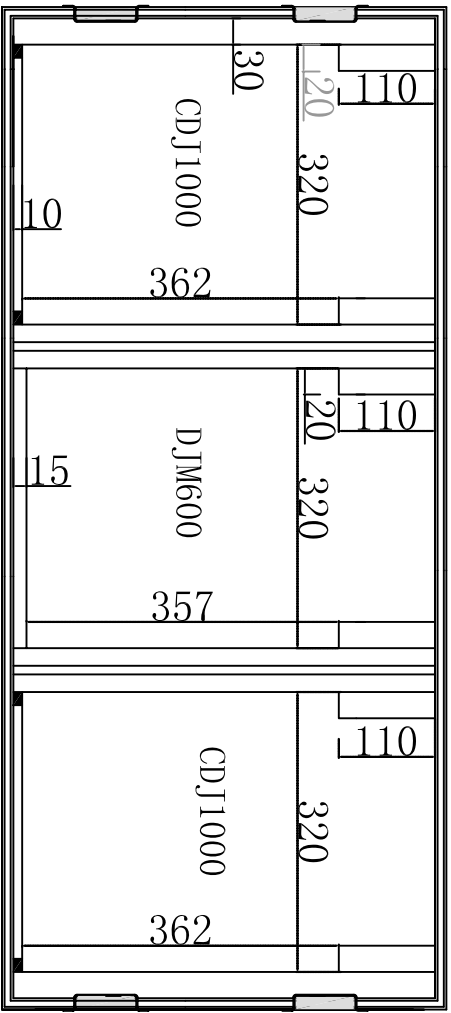
Top View
