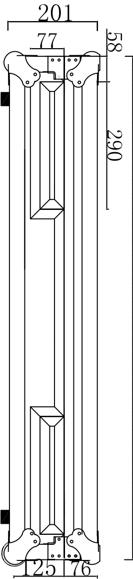
Front View
