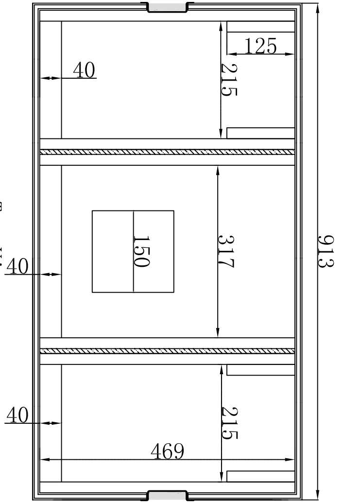
Top View
